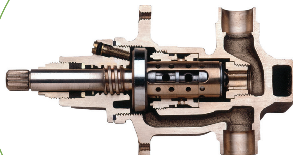
Temptrol® pressure-balancing shower valve
